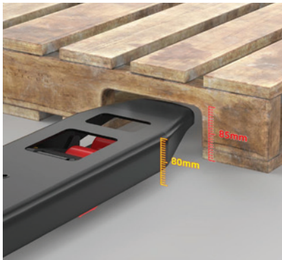
Unique fork design to ensure pallet entry and exit.
